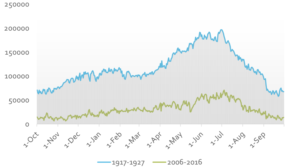
Columbia River at Priest Rapids Daily Flow Standard Deviation
