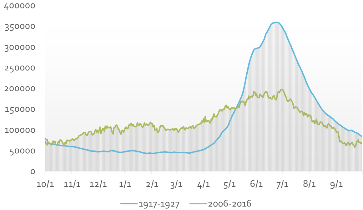
Columbia River at Priest Rapids Daily Flow Average
