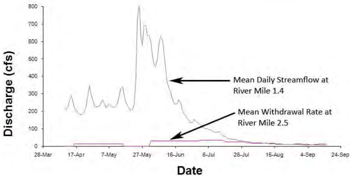
Figure 23. Plot of mean daily streamflow and mean withdrawal rate for Peshastin Creek for part of the year in 2003. High flows are proportionally less affected by withdrawal than low flows.
