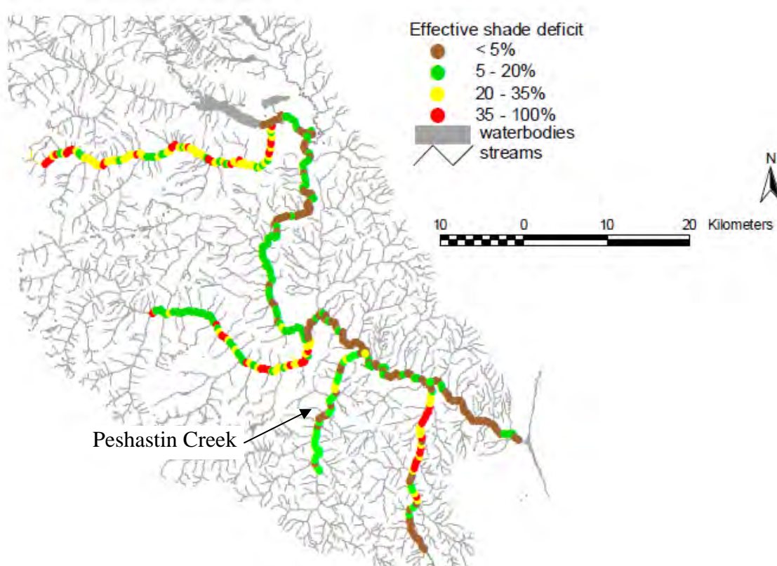
Figure 54. Effective shade deficit in the Wenatchee River basin. Reproduced from WDOE (2005).
