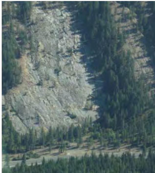
Figure 3. Low elevation aerial photograph of a large Chumstick Formation outcrop on a northwest facing slope of a hogback ridge near river mile 5.9. Sandstone outcrops such as this can contribute fine sediment to the channel over time.
