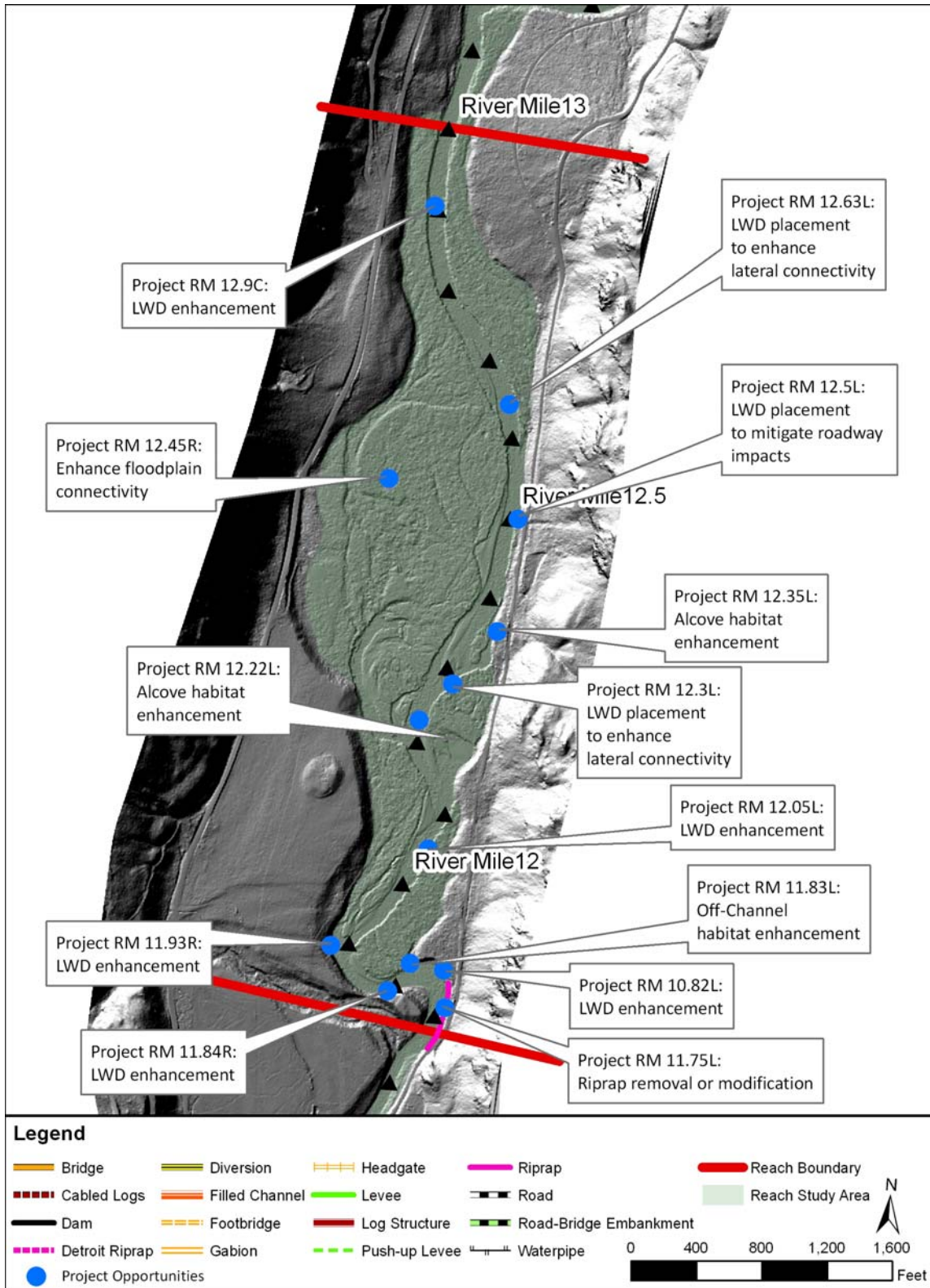
Figure 34. LiDAR hillshade of reach C5a illustrating topography in relation to human features and project locations in the reach. Flow is from north to south.
