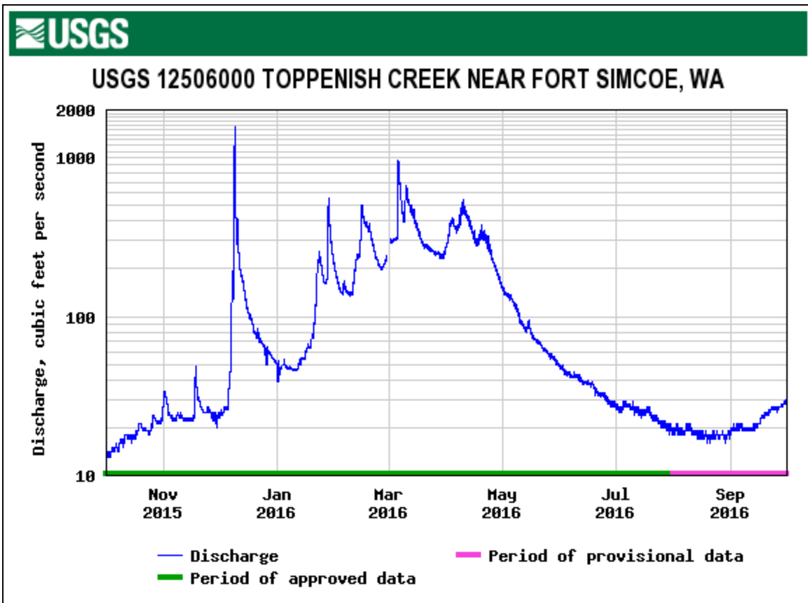
Figure 1. Hydrograph on Toppenish Creek at river mile 40 for Water Year 2016.
