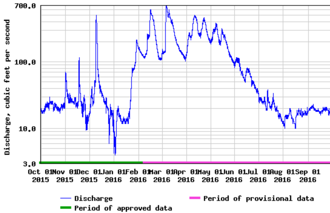
Figure 2. Hydrograph on Ahtanum Creek near the mouth for Water Year 2016.
